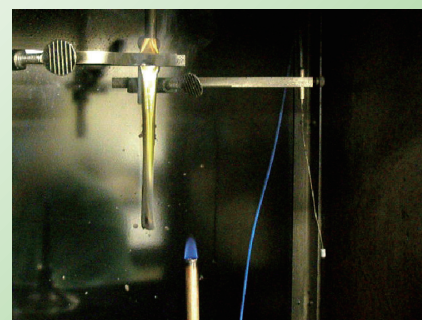
2 回目着火 Second ignition
