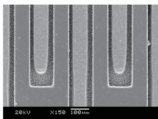
0.2mm Pitch / Clearance 10μm
