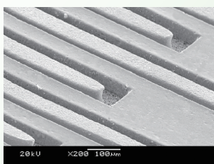
0.2mm Pitch / Clearance 10μm
